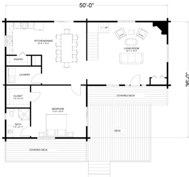
MAIN FLOOR 1435 SQ FT
