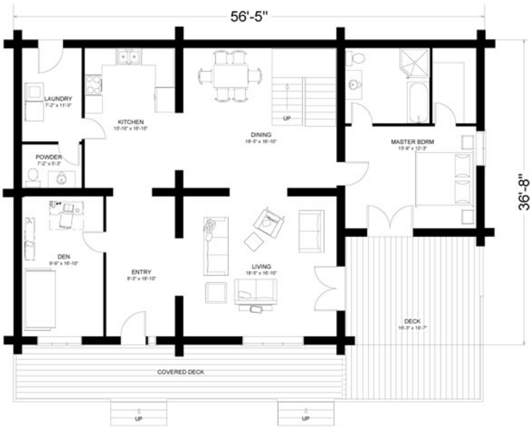
MAIN FLOOR 1850 SQ FT
