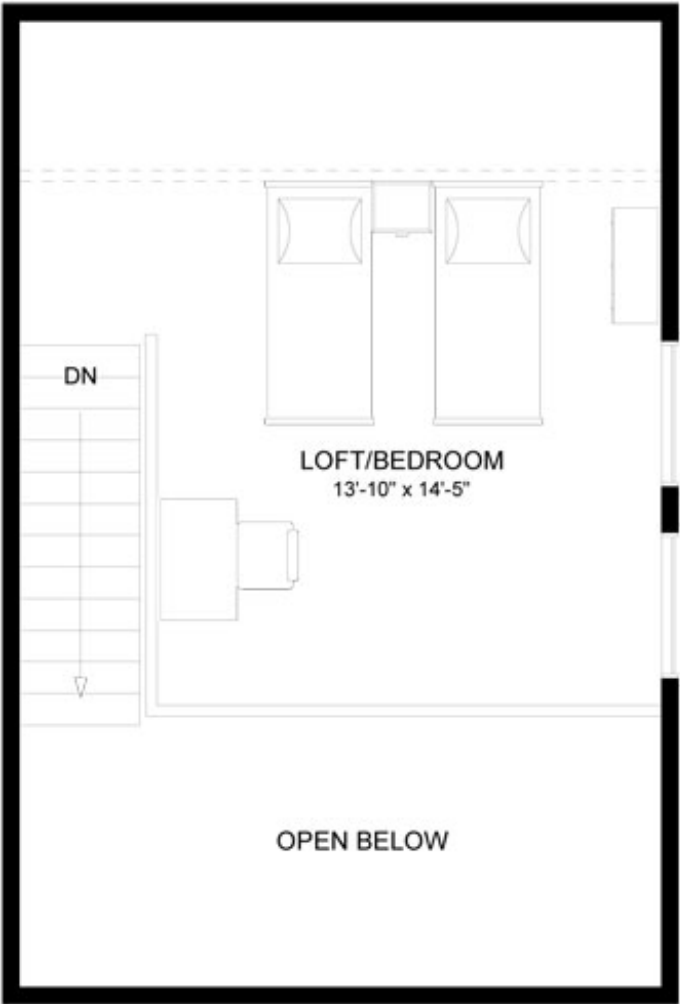
SECOND FLOOR 230 SQ FT
