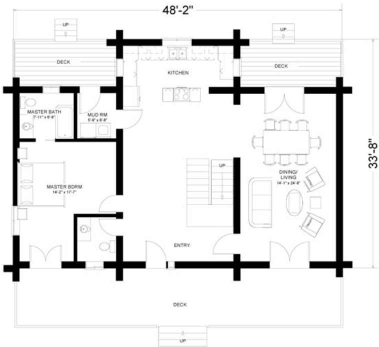
MAIN FLOOR 1418 SQ FT
