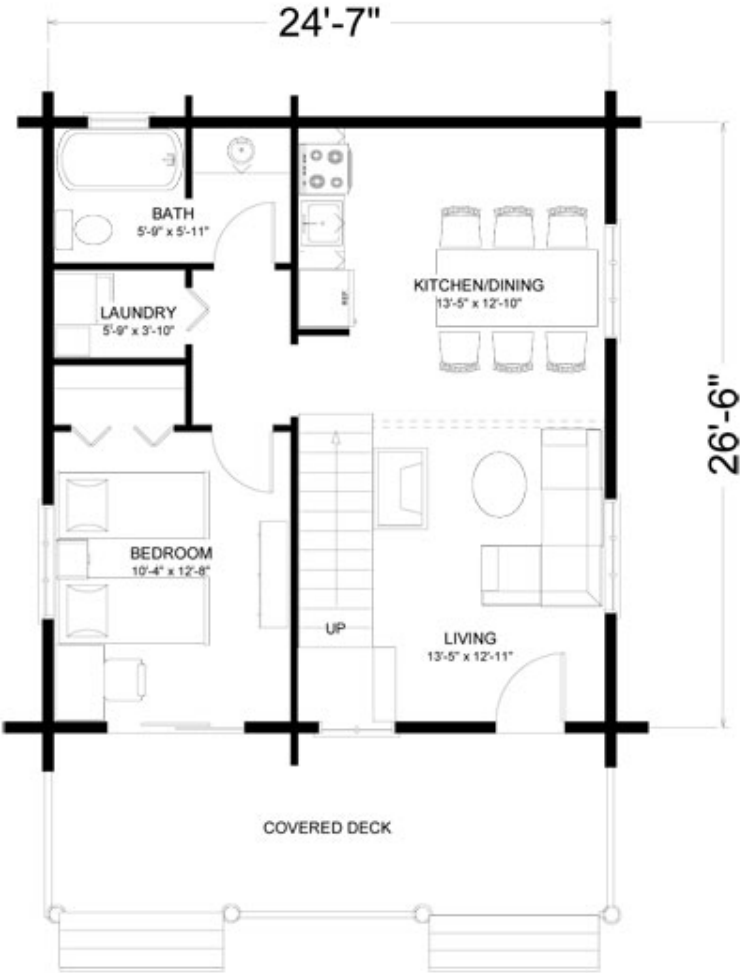
MAIN FLOOR 680 SQ FT
