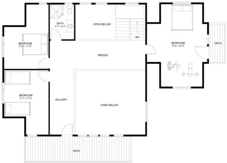
SECOND FLOOR 1135 SQ FT
