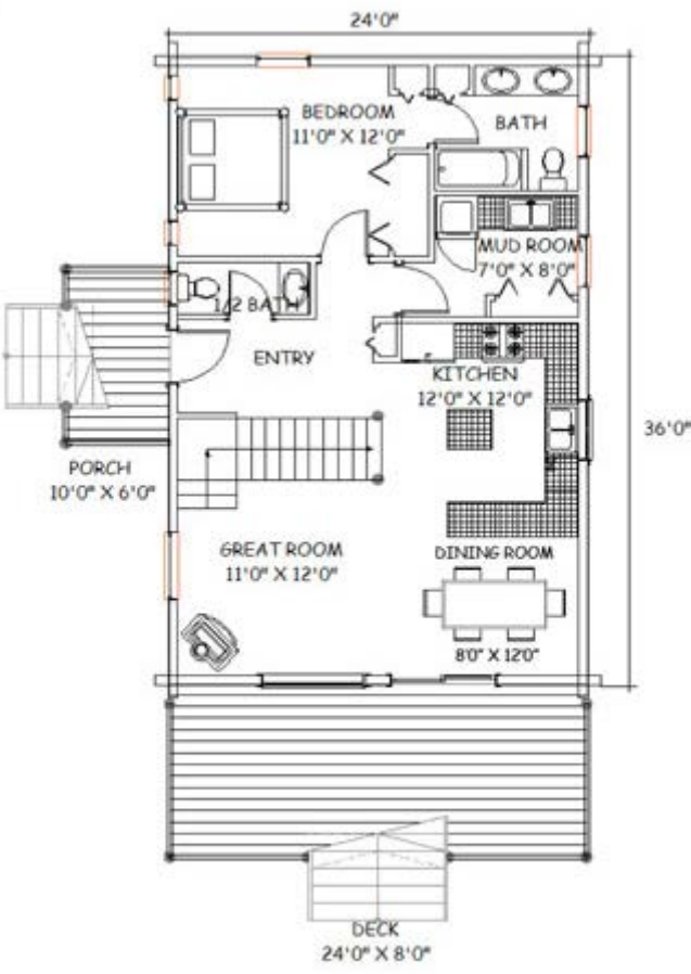
MAIN FLOOR: 864 SQ. FT.
